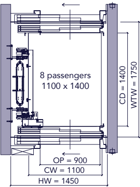
Two entrances 180°, car frame at the side
