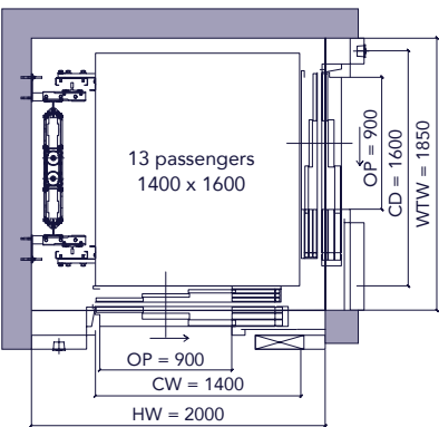
Two entrances 90°, car frame at the side
