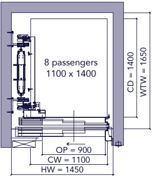
One entrance, car frame at the side
